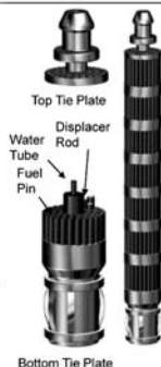
AHWR Fuel assembly
